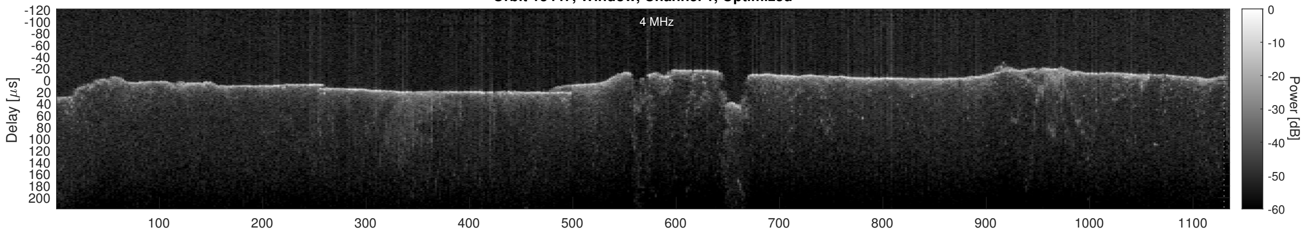
Orbit 13447, Cluttergram
