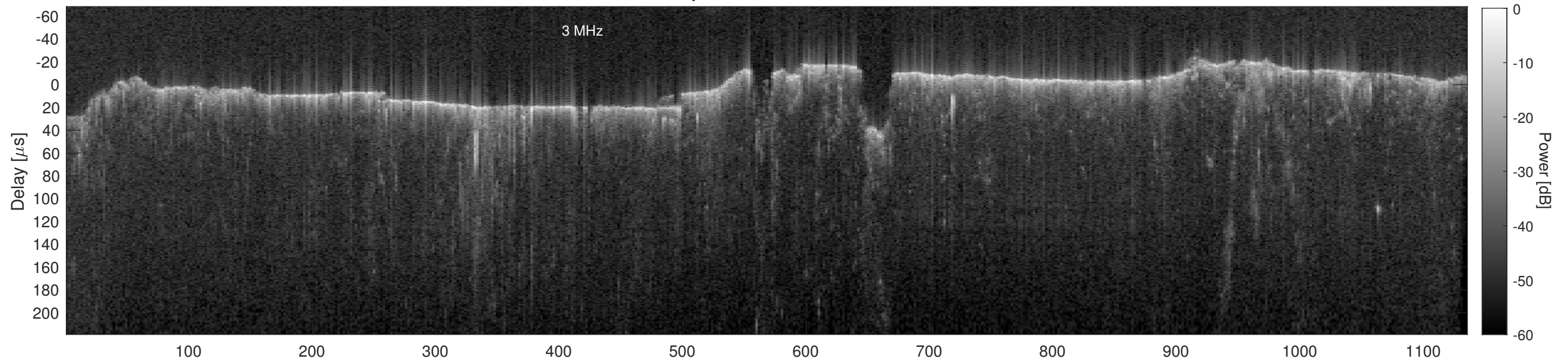
Orbit 13447, Cluttergram
