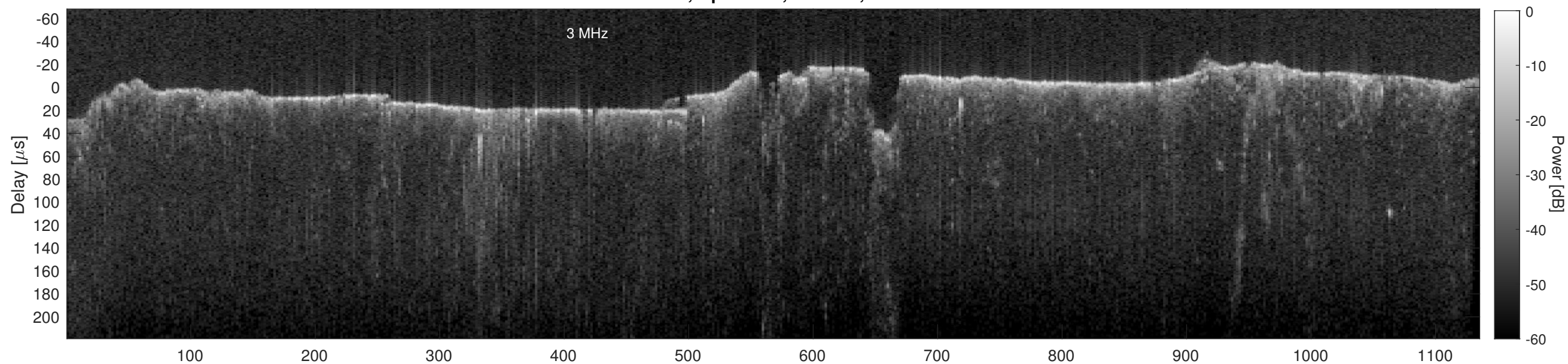
Orbit 13447, Cluttergram
