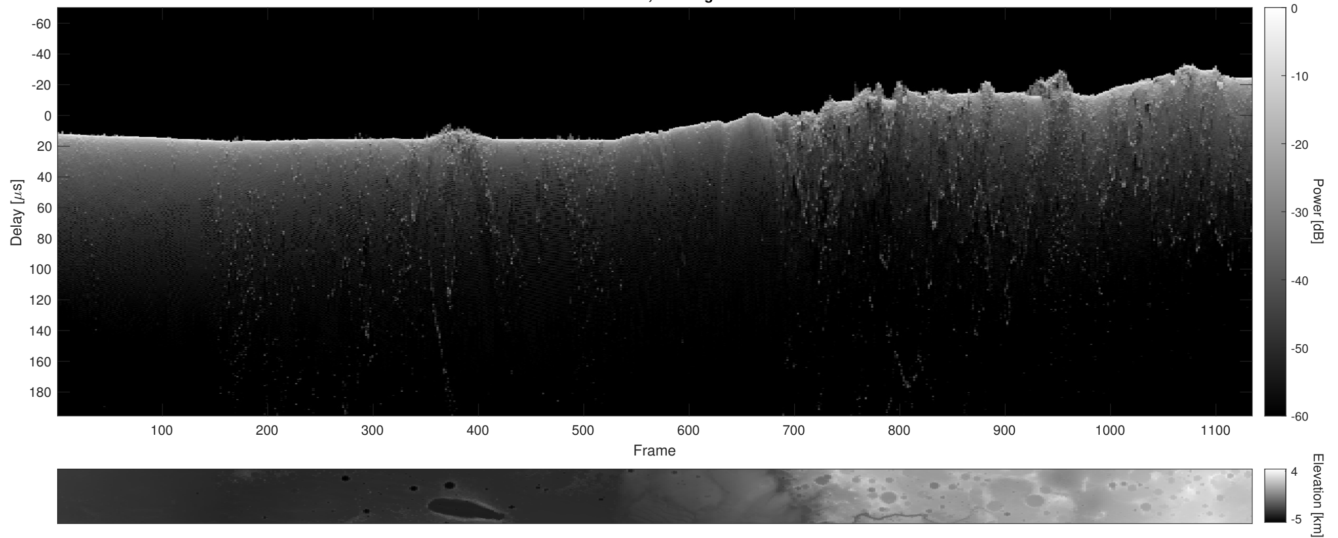
Orbit 13448, Cluttergram
