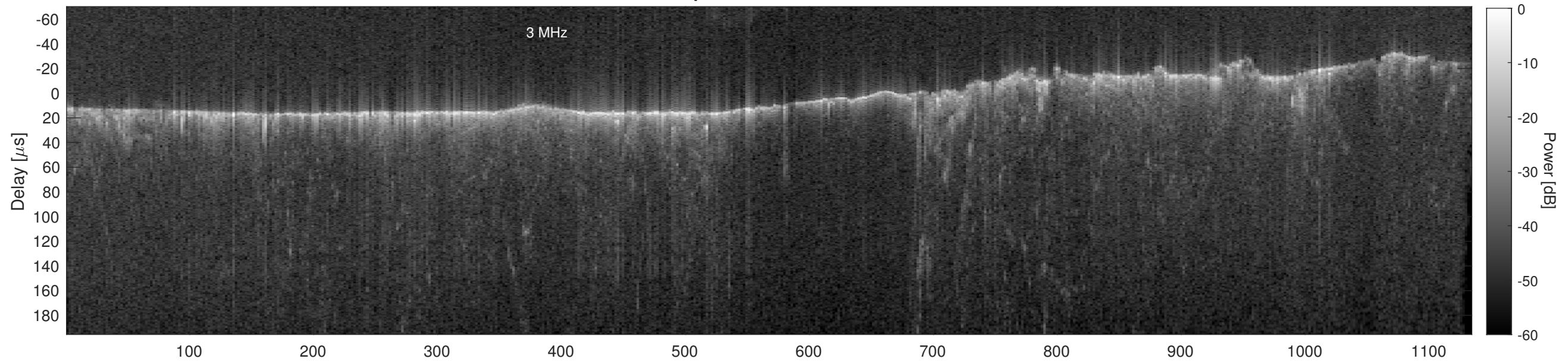
Orbit 13448, Cluttergram
