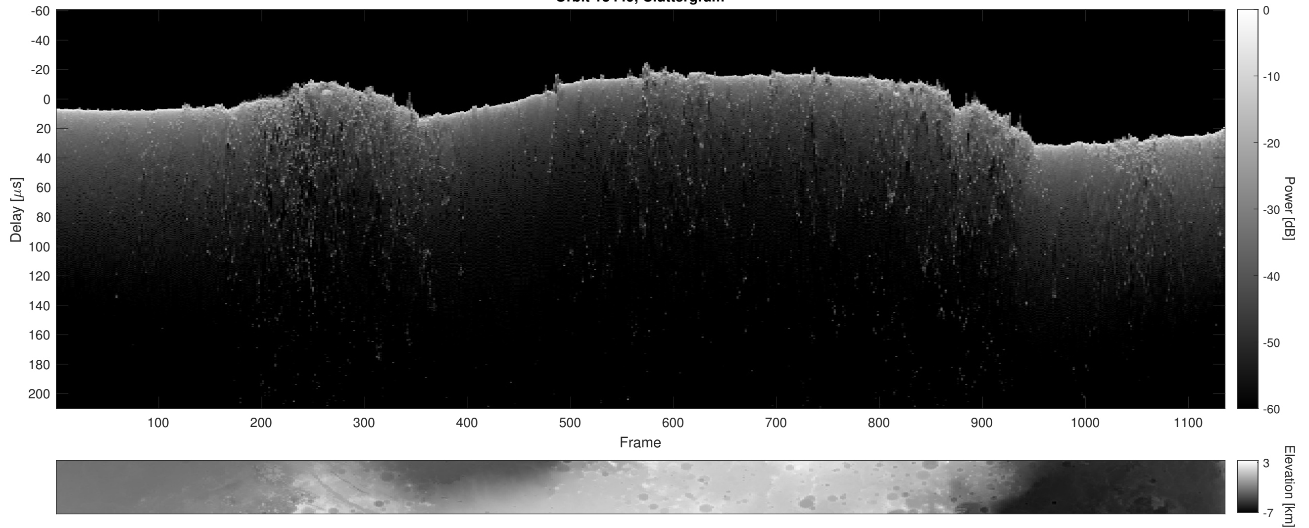
Orbit 13449, Cluttergram
