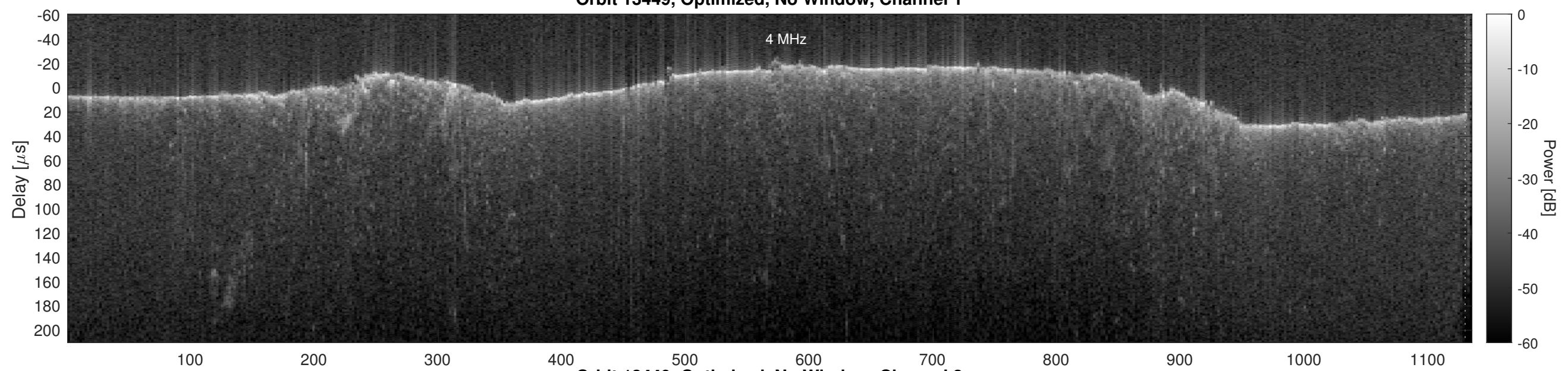
Orbit 13449, Optimized, No Window, Channel 2
