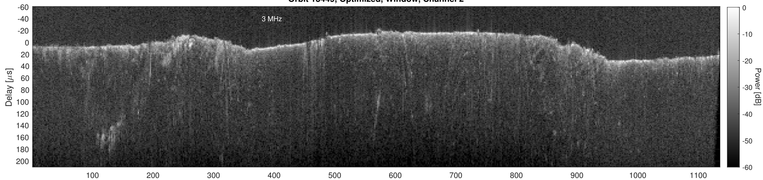
Orbit 13449, Cluttergram
