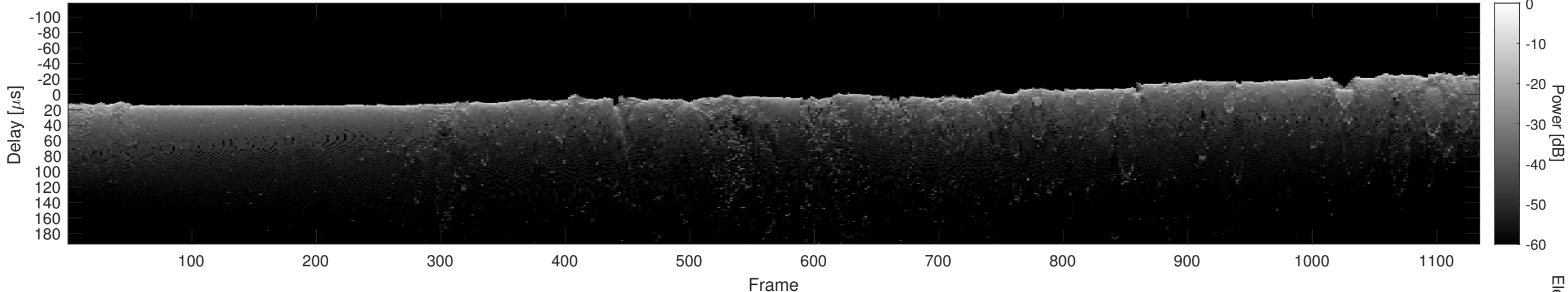
Orbit 13450, Cluttergram
