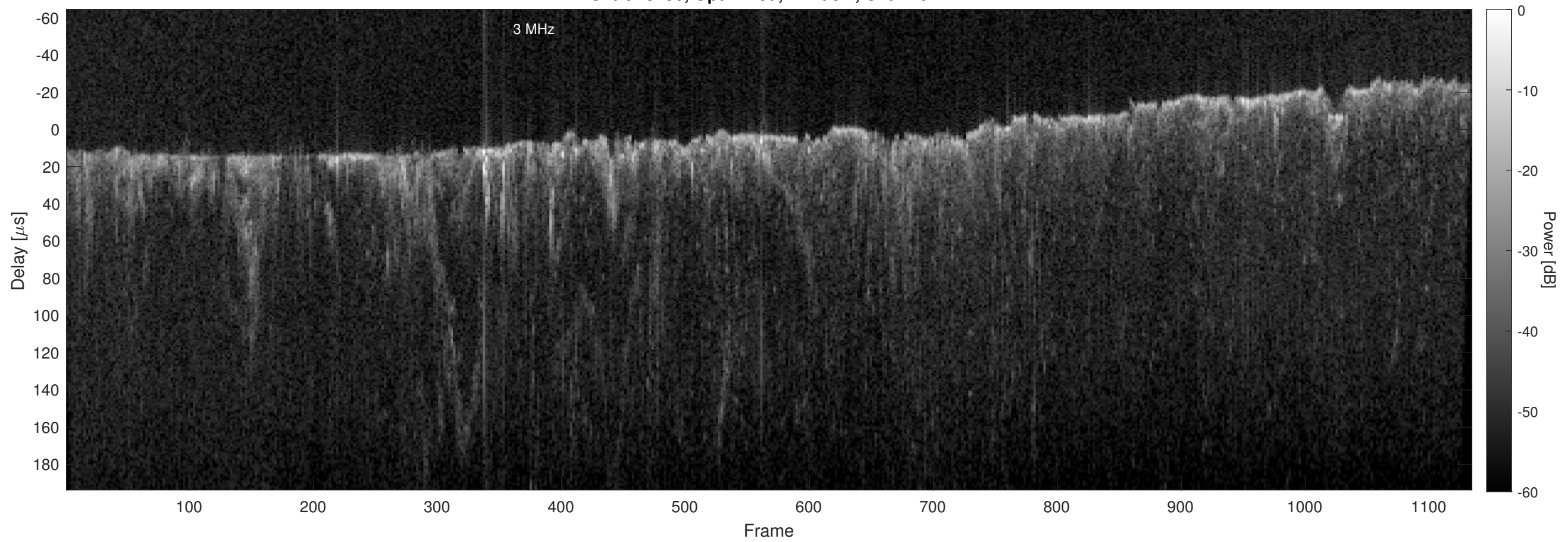
Orbit 13450, Optimized, Window, Channel 2
