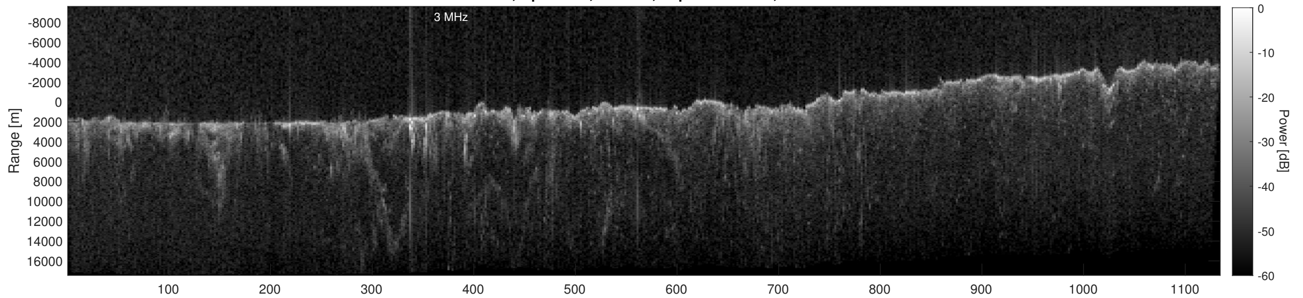
Orbit 13450, Depth-Corrected Cluttergram
