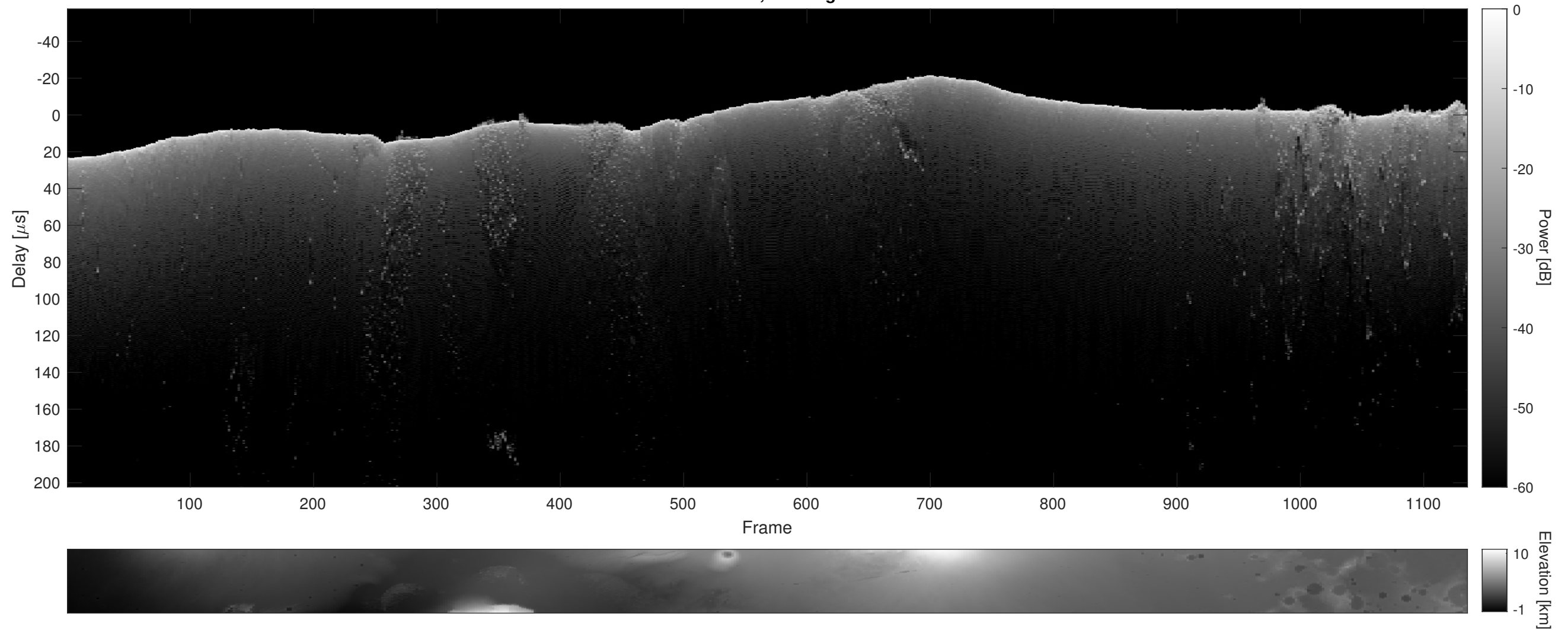
Orbit 13451, Cluttergram
