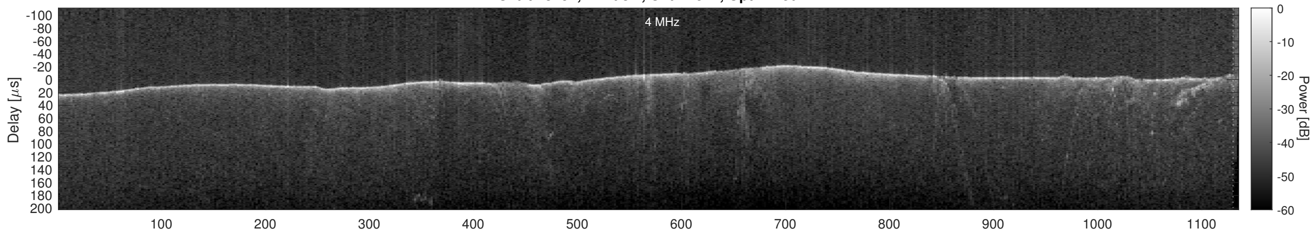
Orbit 13451, Cluttergram
