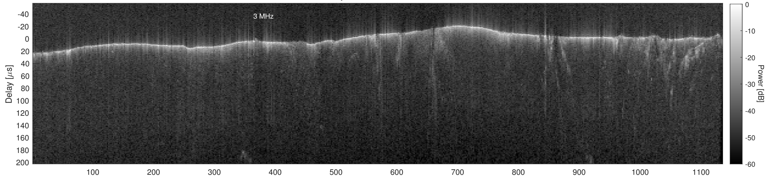
Orbit 13451, Cluttergram
