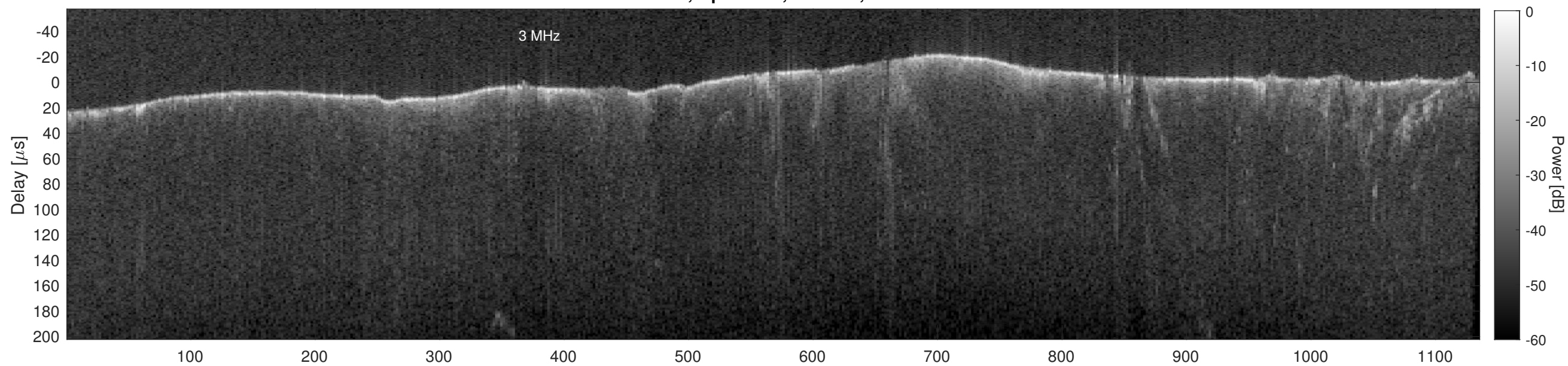
Orbit 13451, Cluttergram
