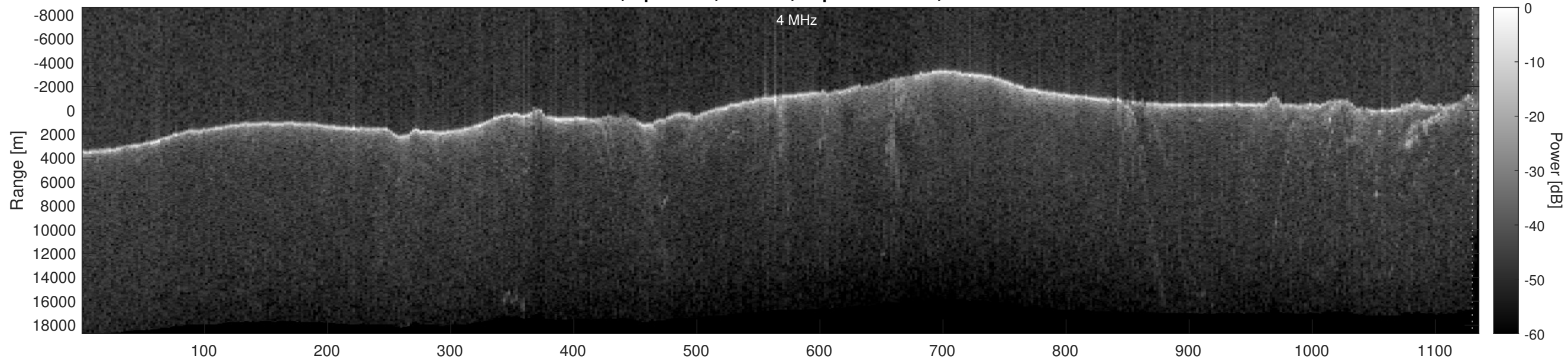
Orbit 13451, Optimized, Window, Depth-Corrected, Channel 2
