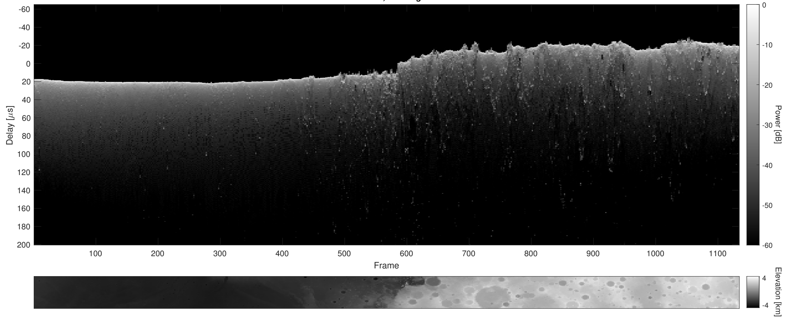
Orbit 13452, Cluttergram
