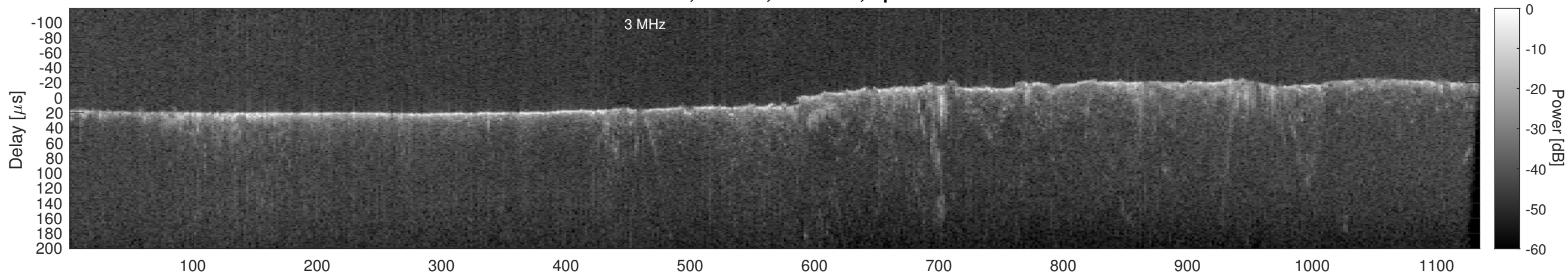
Orbit 13452, Cluttergram
