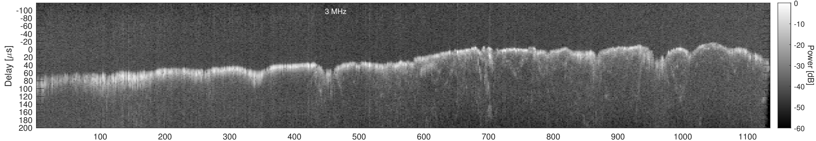
Orbit 13452, Window, Channel 2, Chapman
