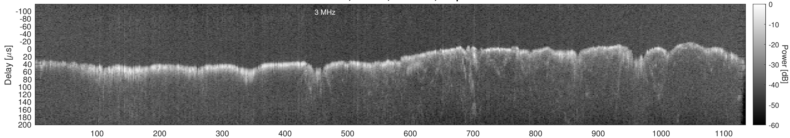
Orbit 13452, Window, Channel 2, Optimized
