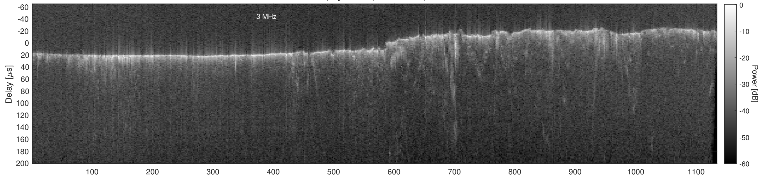
Orbit 13452, Cluttergram
