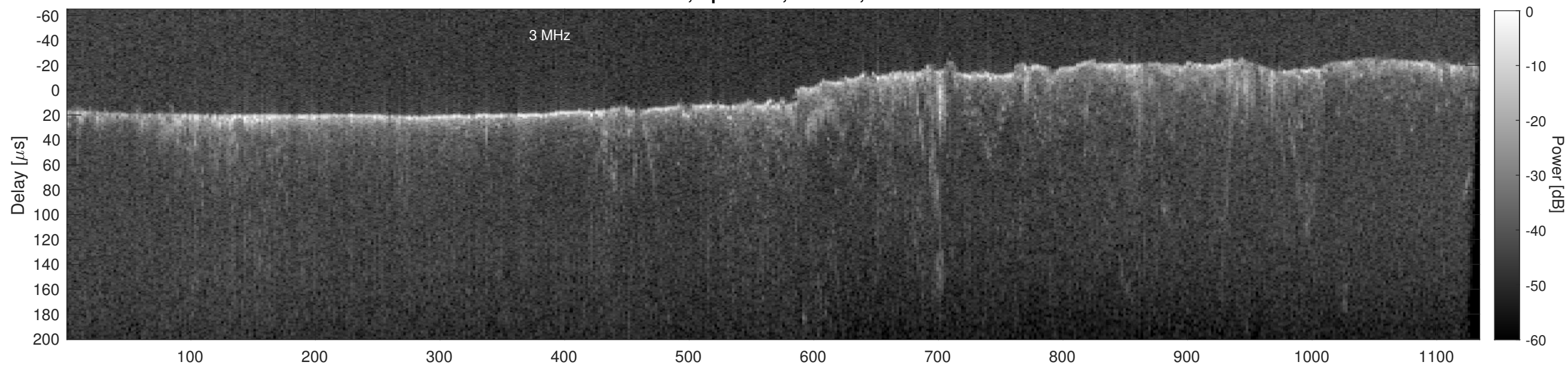
Orbit 13452, Cluttergram
