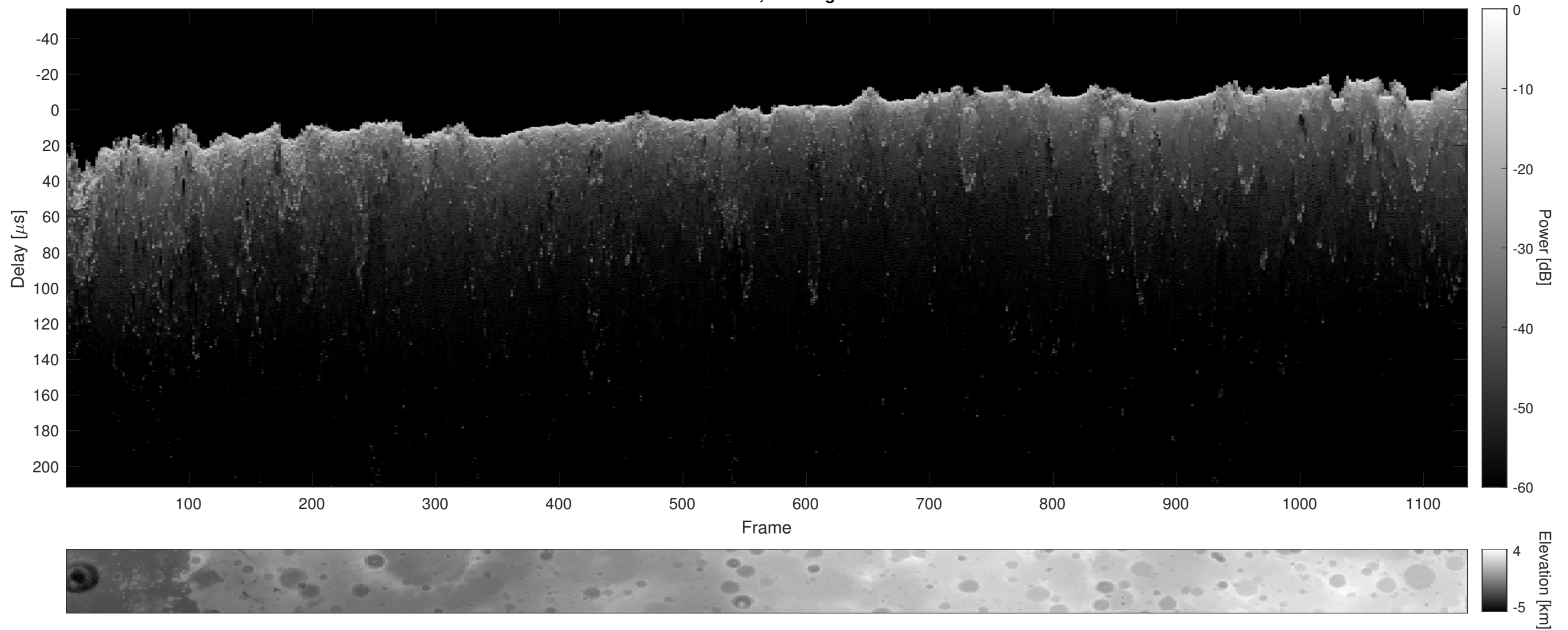
Orbit 13453, Cluttergram
