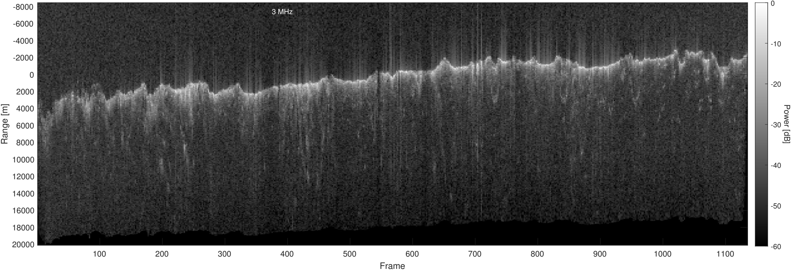
Orbit 13453, Optimized, No Window, Depth-Corrected, Channel 2
