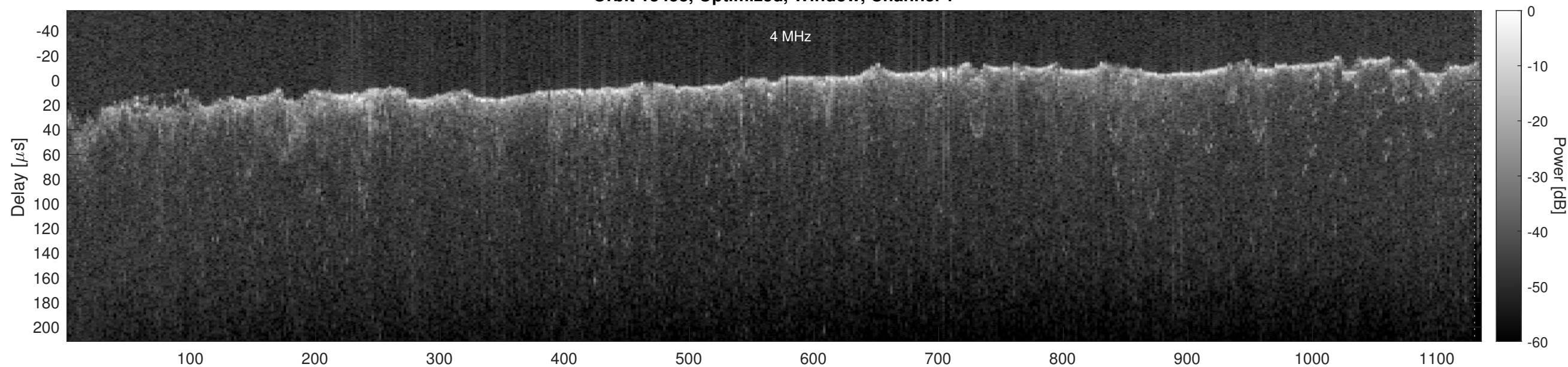
Orbit 13453, Optimized, Window, Channel 2
