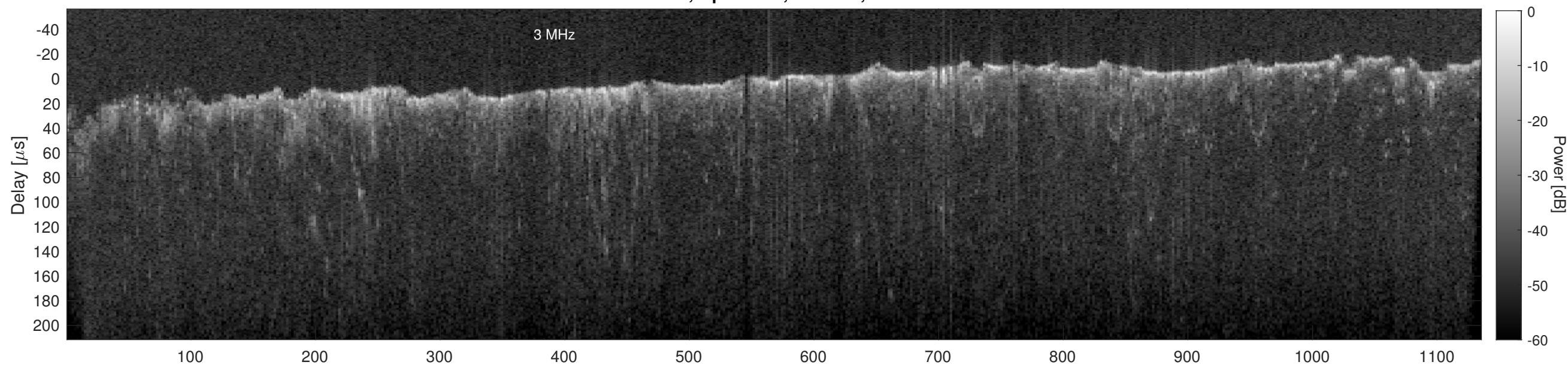
Orbit 13453, Cluttergram
