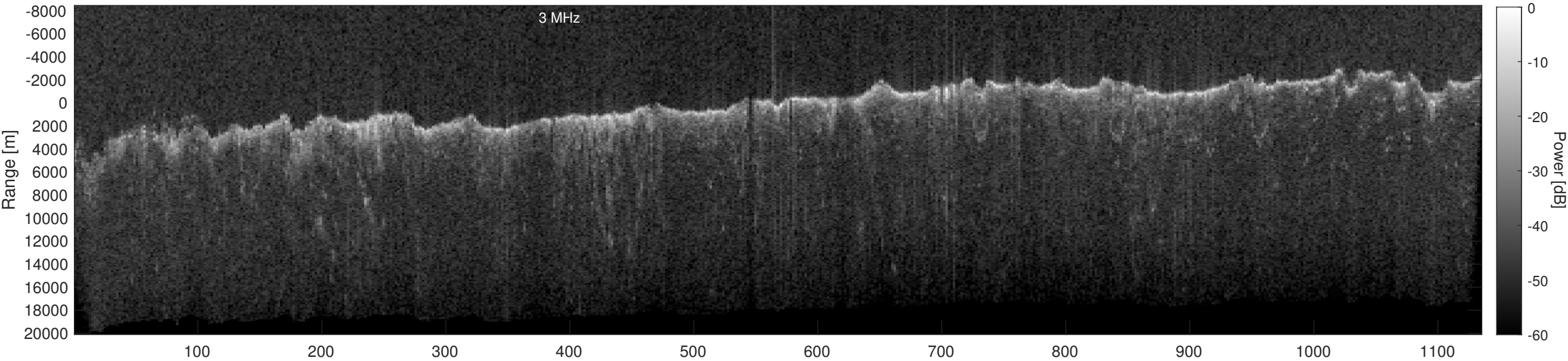
Orbit 13453, Depth-Corrected Cluttergram
