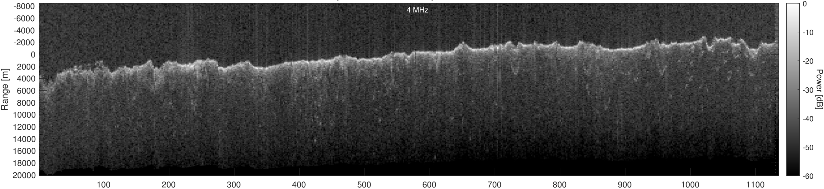
Orbit 13453, Optimized, Window, Depth-Corrected, Channel 2
