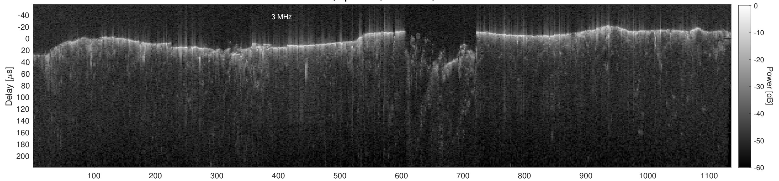
Orbit 13454, Cluttergram
