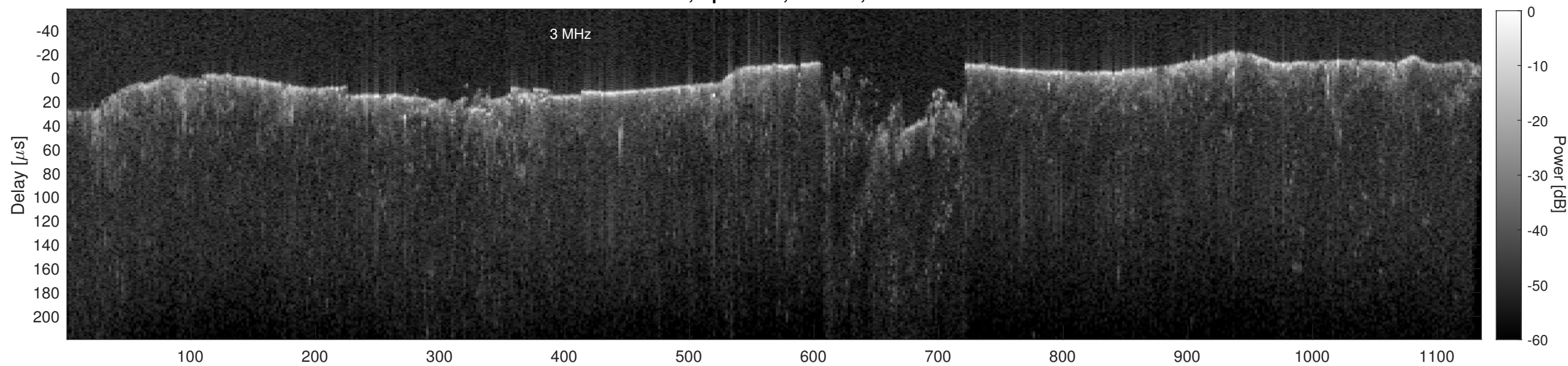
Orbit 13454, Cluttergram
