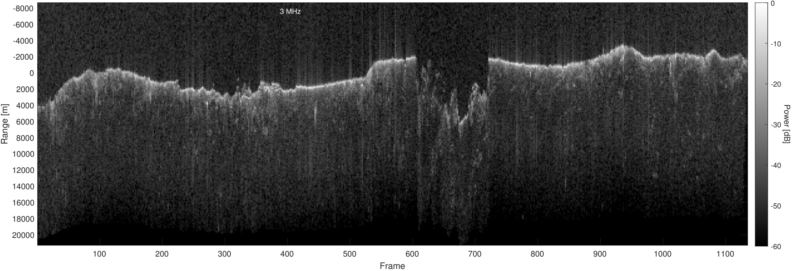
Orbit 13454, Optimized, Window, Depth-Corrected, Channel 2
