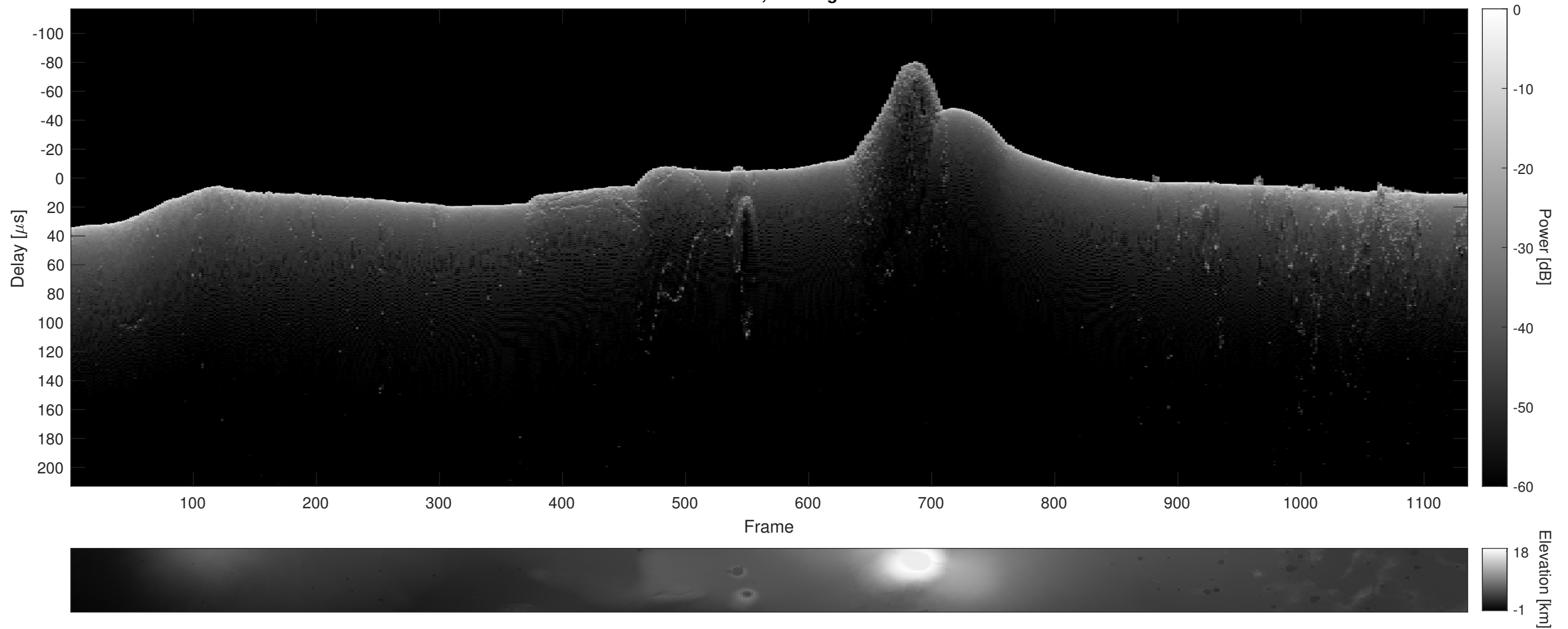
Orbit 13458, Cluttergram
