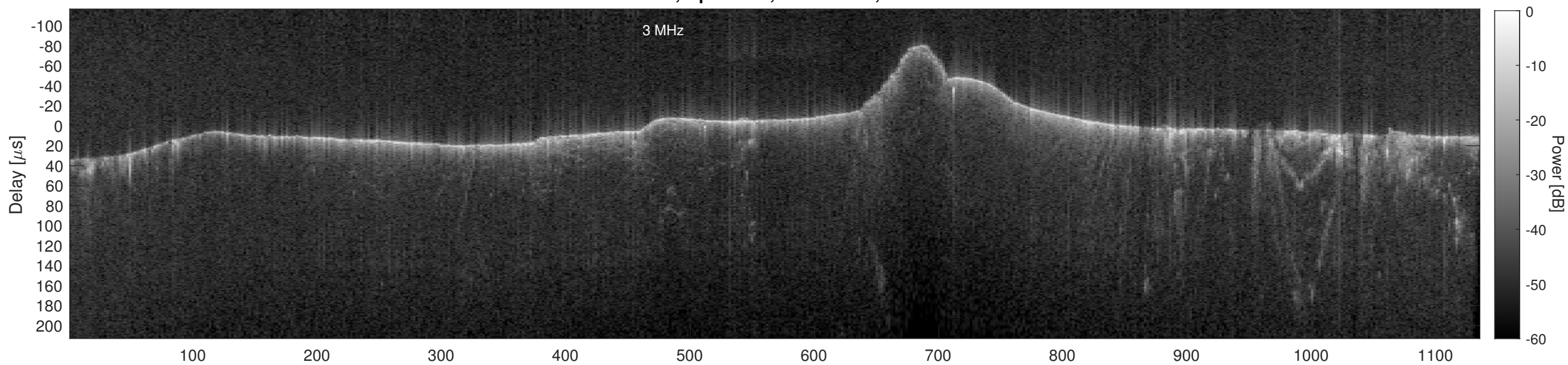
Orbit 13458, Cluttergram
