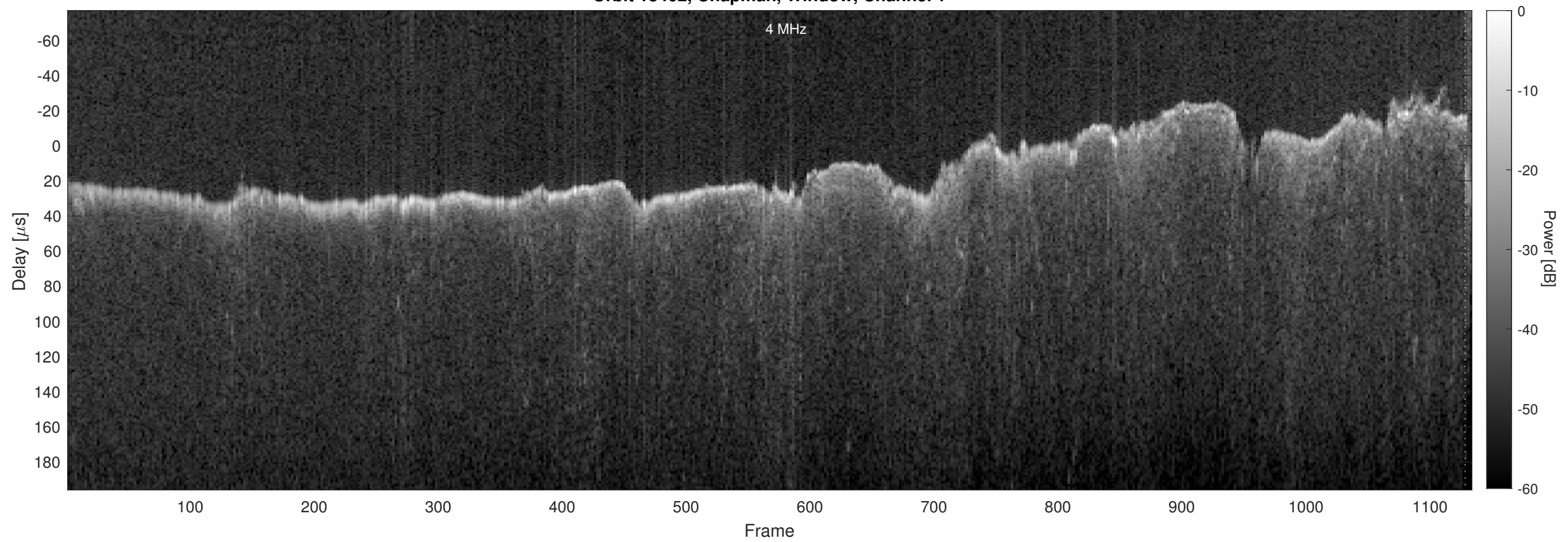
Orbit 13462, Chapman, Window, Channel 2
