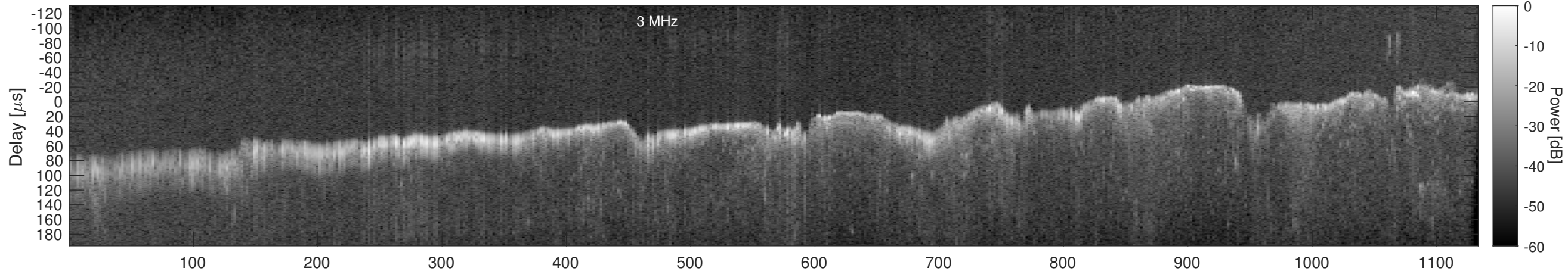
Orbit 13462, Window, Channel 2, Chapman
