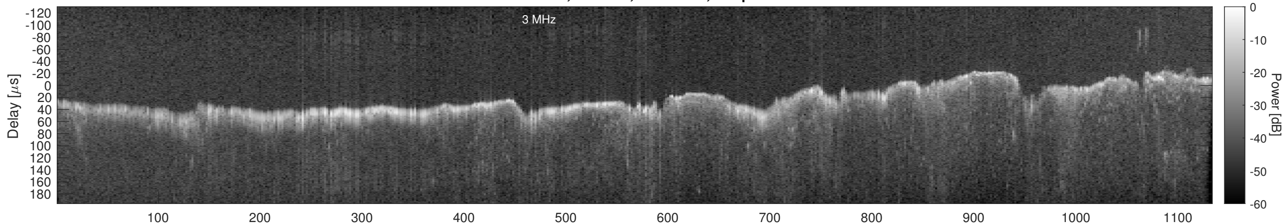
Orbit 13462, Window, Channel 2, Optimized
