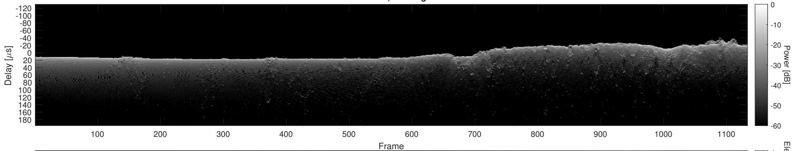
Orbit 13462, Cluttergram
