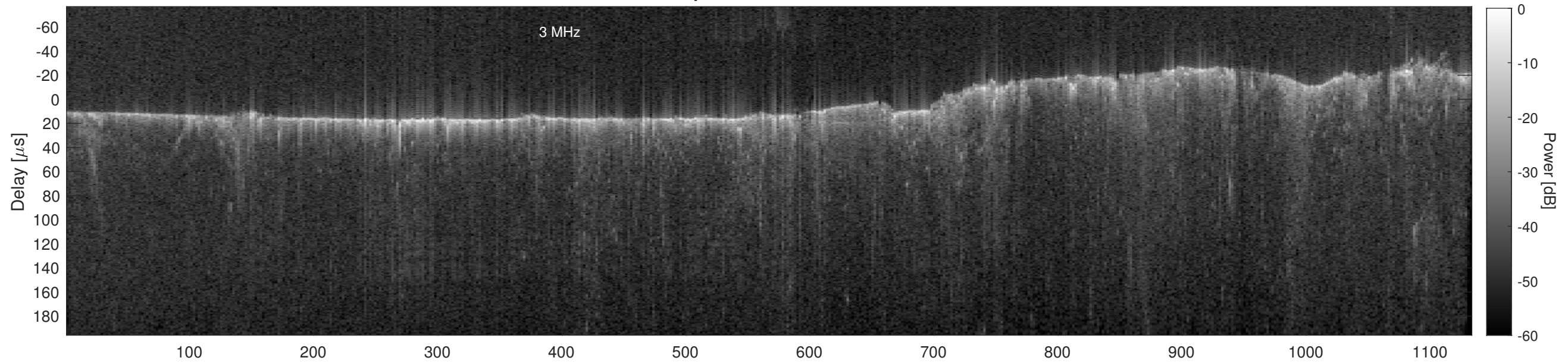
Orbit 13462, Cluttergram
