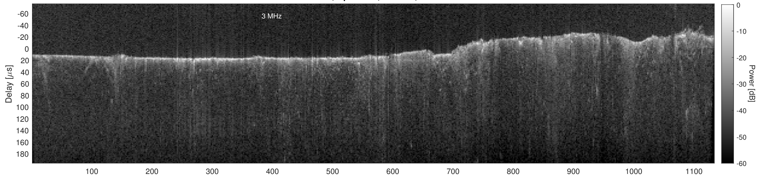
Orbit 13462, Cluttergram
