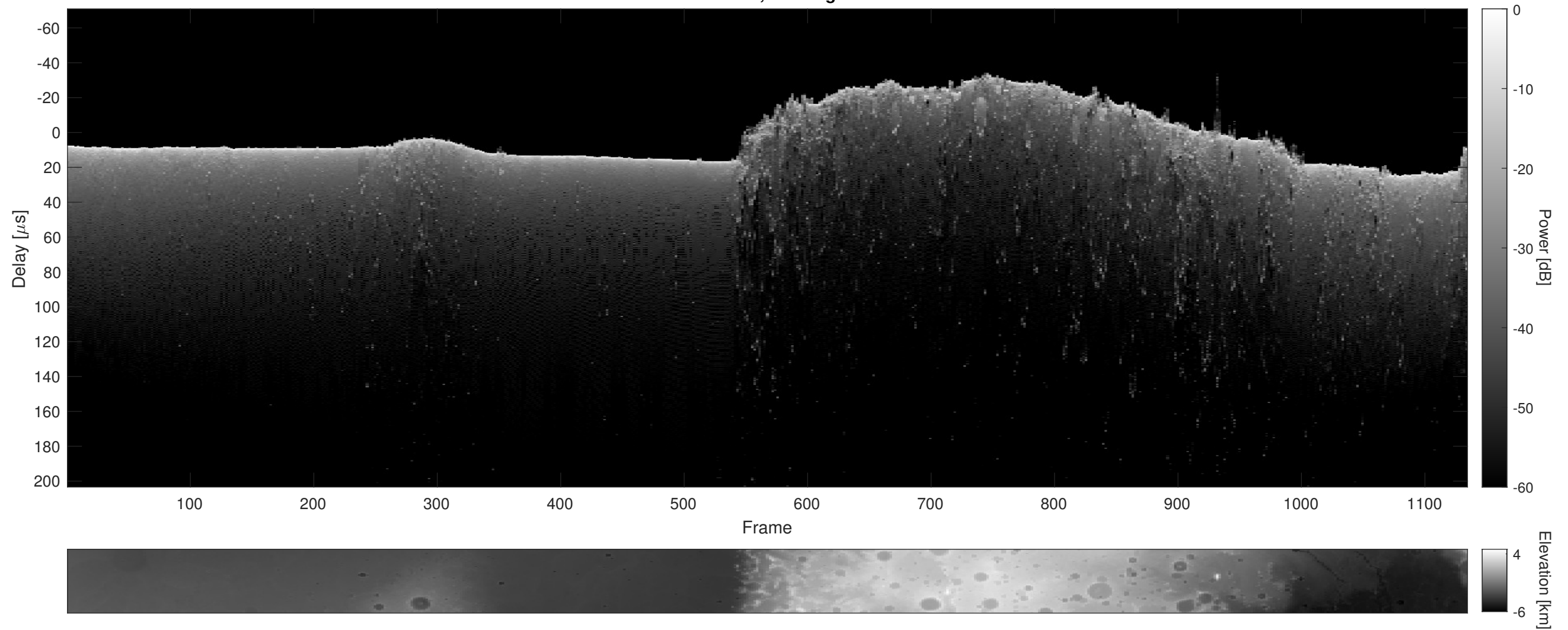
Orbit 13463, Cluttergram
