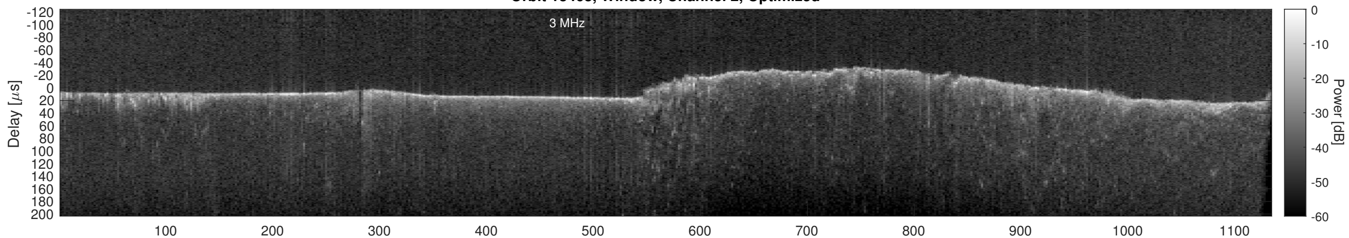
Orbit 13463, Cluttergram
