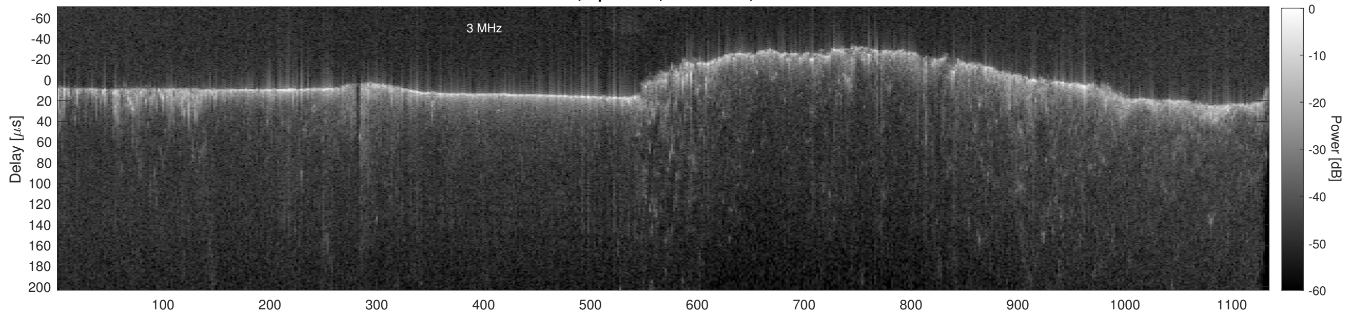
Orbit 13463, Cluttergram
