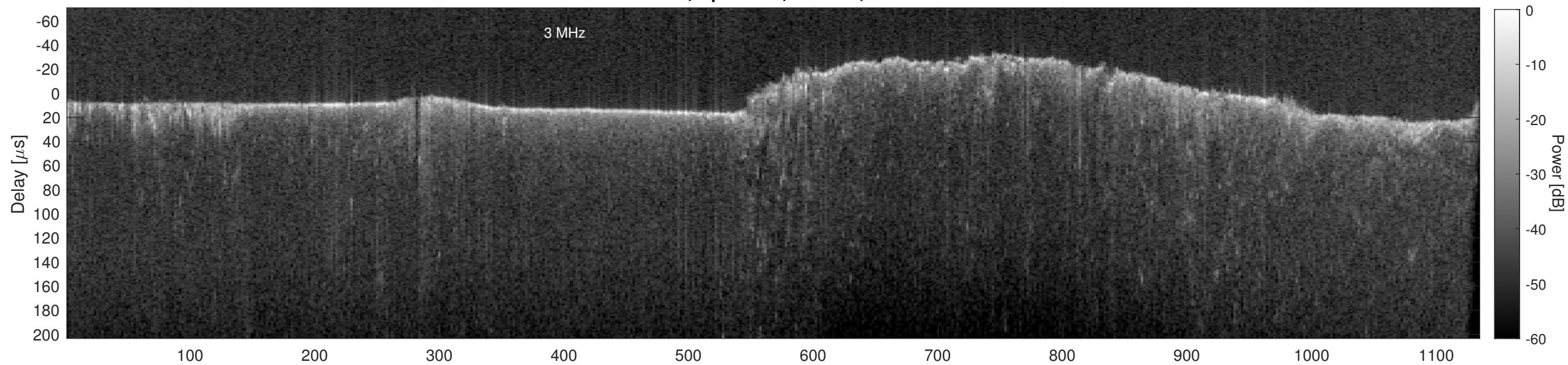
Orbit 13463, Cluttergram
