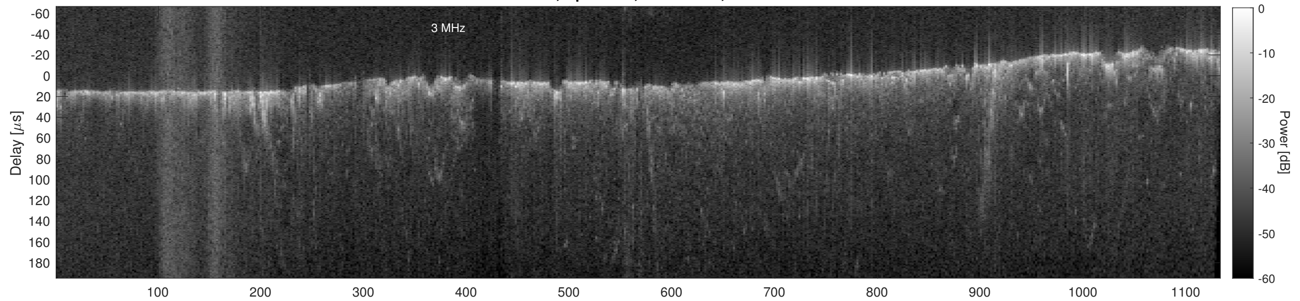
Orbit 13464, Cluttergram
