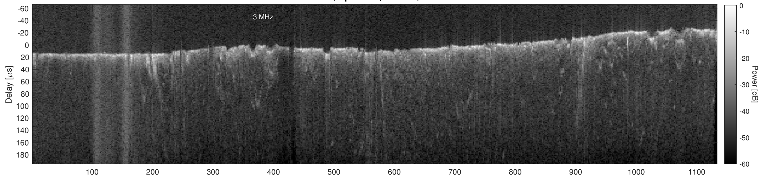
Orbit 13464, Cluttergram
