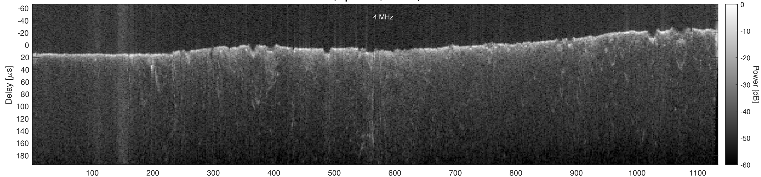
Orbit 13464, Optimized, Window, Channel 2
