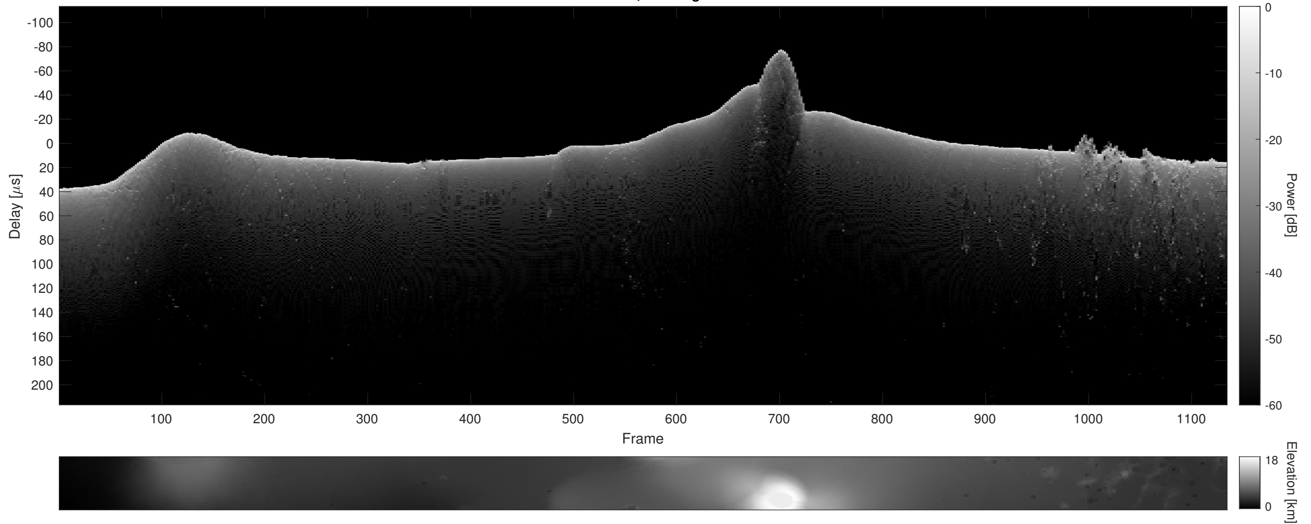
Orbit 13465, Cluttergram
