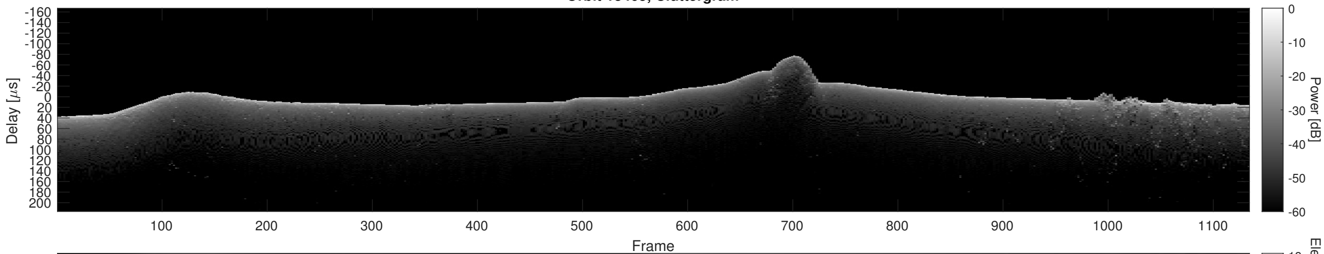
Orbit 13465, Cluttergram
