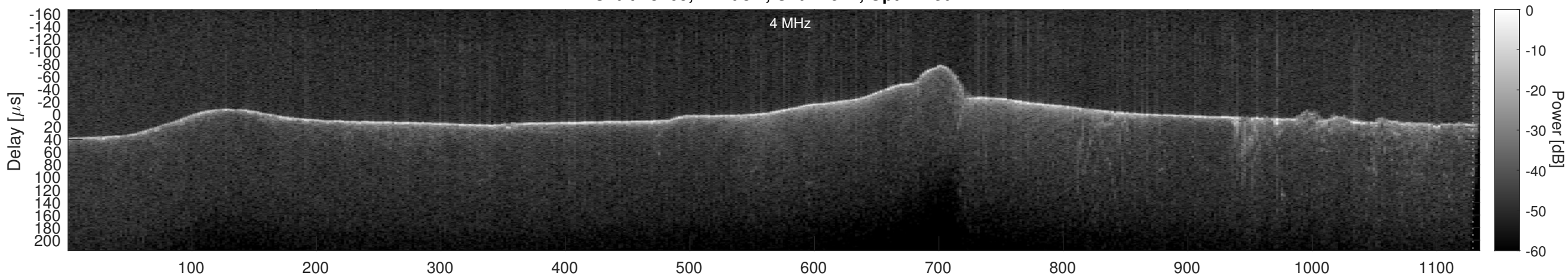
Orbit 13465, Cluttergram
