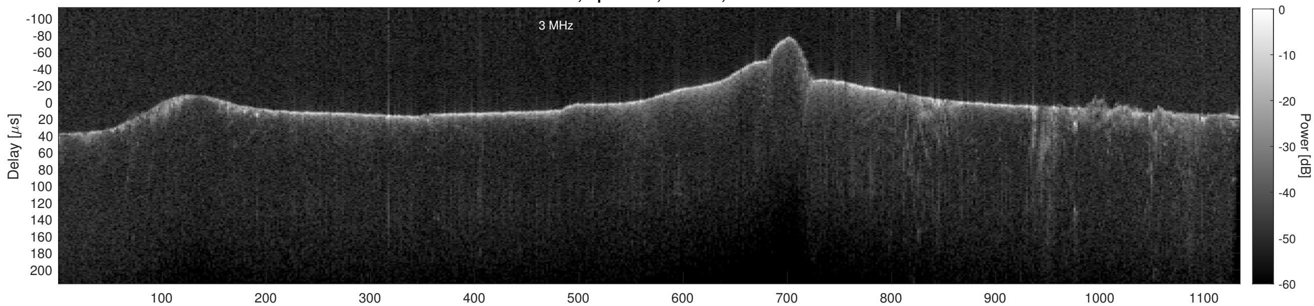
Orbit 13465, Cluttergram
