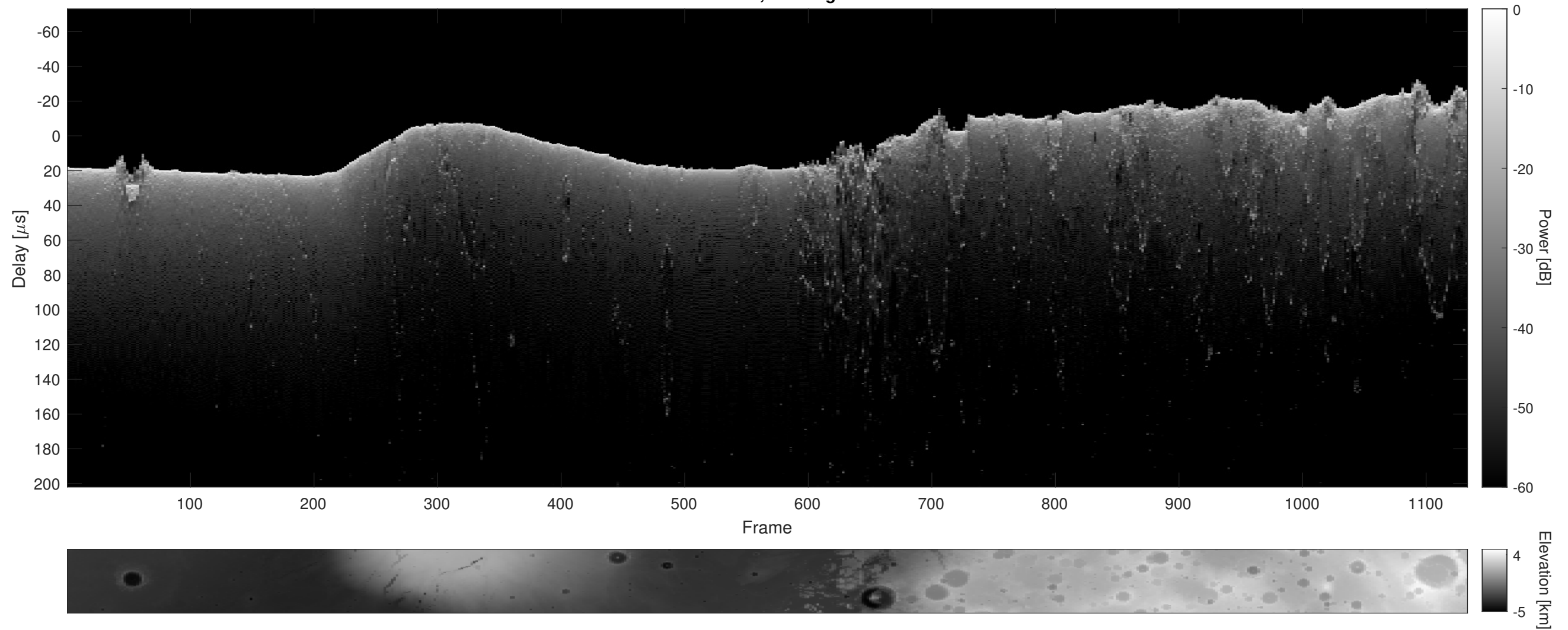
Orbit 13466, Cluttergram
