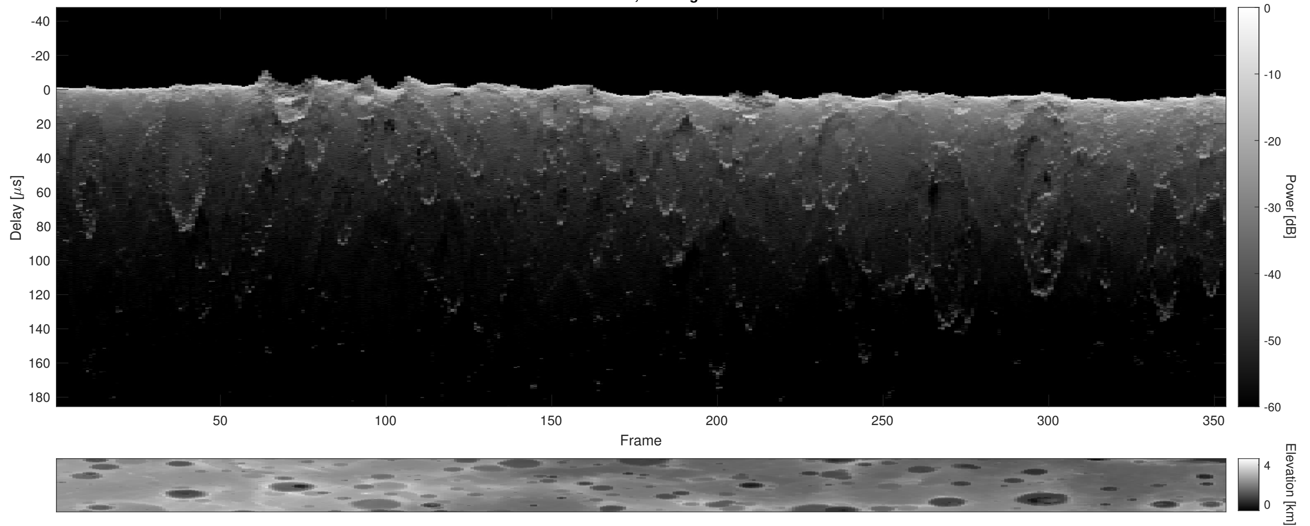
Orbit 13467, Cluttergram
