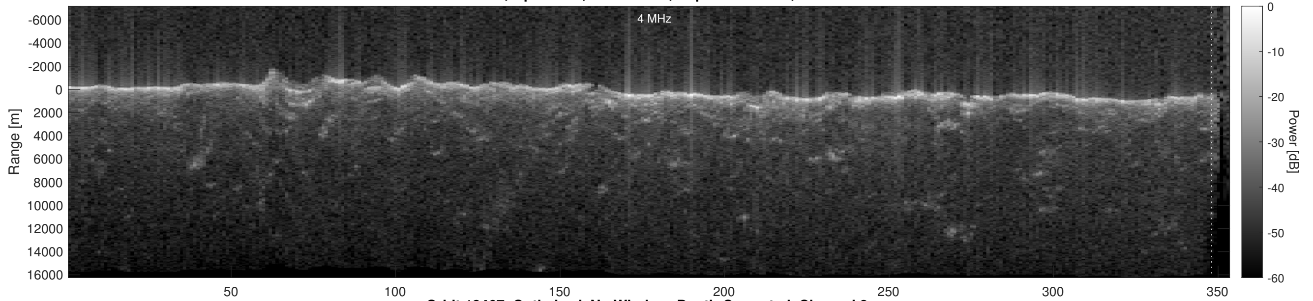
Orbit 13467, Optimized, No Window, Depth-Corrected, Channel 2
