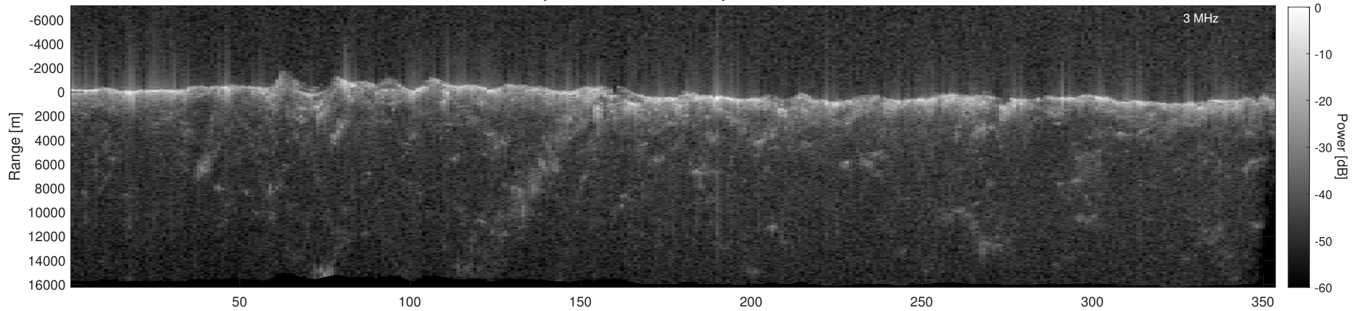
Orbit 13467, Depth-Corrected Cluttergram
