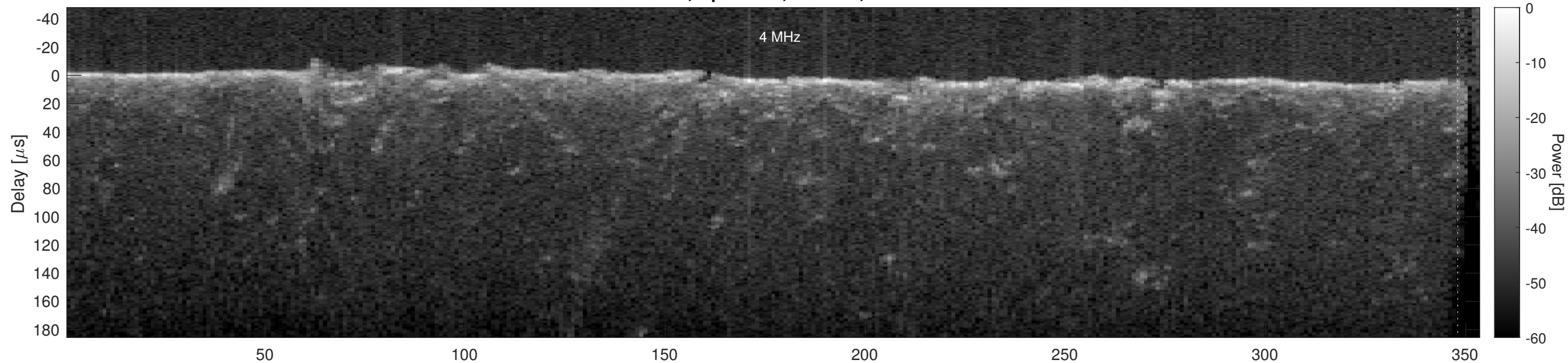
Orbit 13467, Optimized, Window, Channel 2
