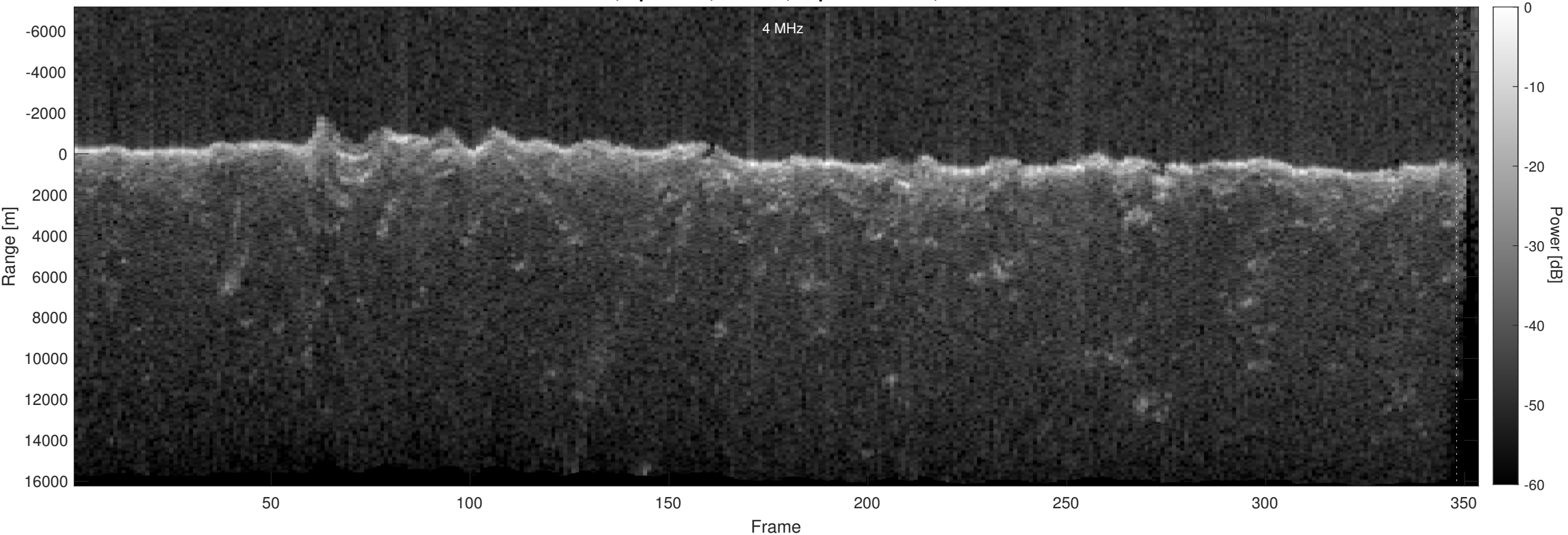
Orbit 13467, Optimized, Window, Depth-Corrected, Channel 2
