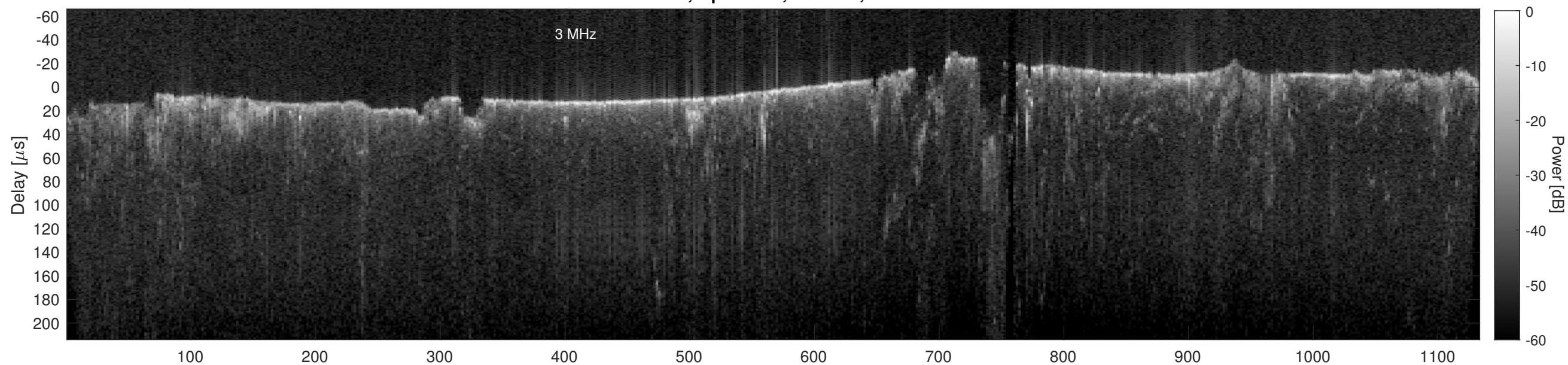
Orbit 13468, Cluttergram
