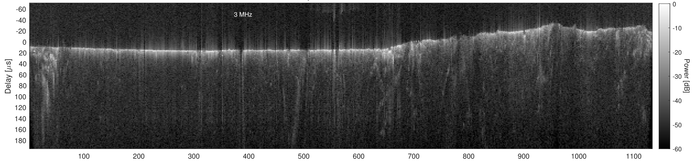
Orbit 13469, Cluttergram
