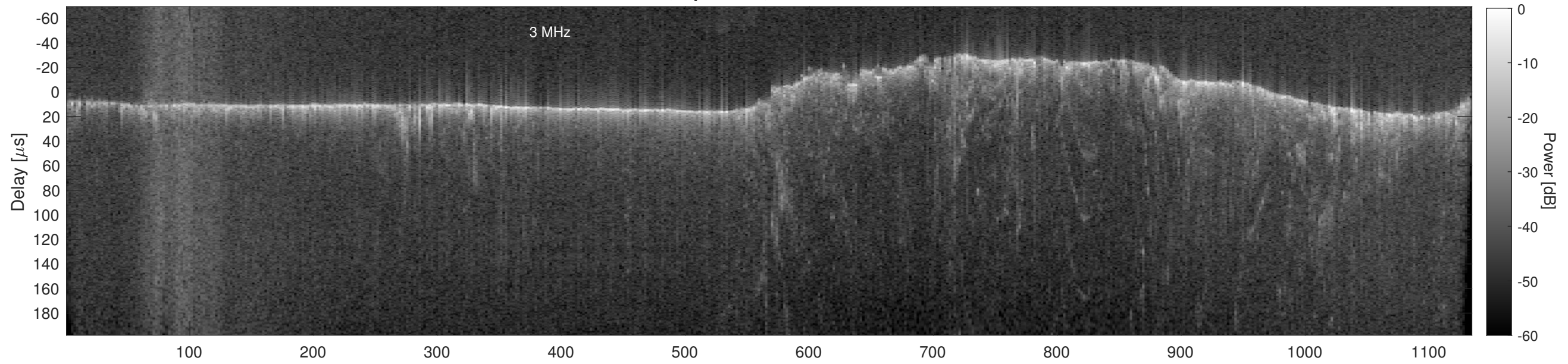
Orbit 13470, Cluttergram
